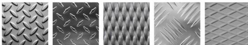
901 rice grain stainless steel AISI-304 902 treadtex stainless steel AISI-316 903 satin stainless steel 5WL AISI-304 (opt. AISI-316) 904 rice grain aluminium 905 striped metal sheet
